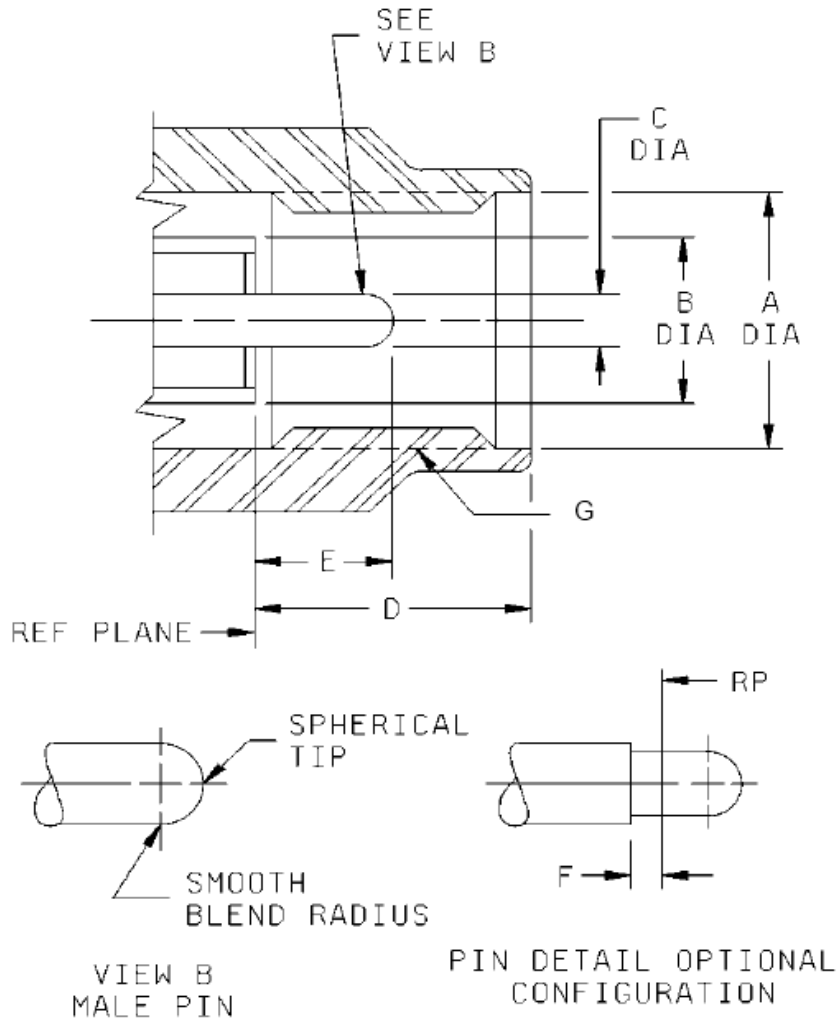
FIGURE 3 (a) – STANDARD TEST CONNECTOR INTERFACE, MALE CONTACT
